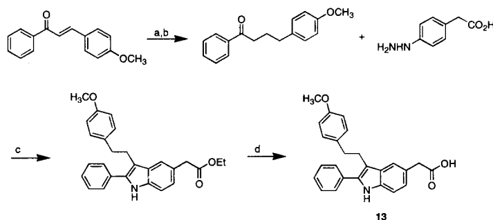
Scheme 1. Reagents and conditions: (a) NaH, (\text{CH}_3)_3\text{SOI} , DMSO, rt, 72%. (b) Zn/ \text{ZnCl}_2 , EtOH, reflux, 85%. (c) \text{ZnCl}_2 , EtOH, reflux, 74%. (d) 1 M NaOH, EtOH, rt, 92%.
